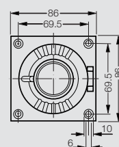
Flange socket
